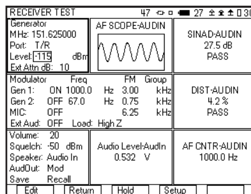
Receiver Test Screen
