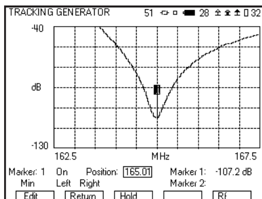
Tracking Generator
