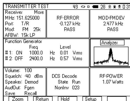
Transmitter Test Screen
