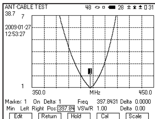
ANT-CABLE Test Screen Showing VSWR Versus Frequency
