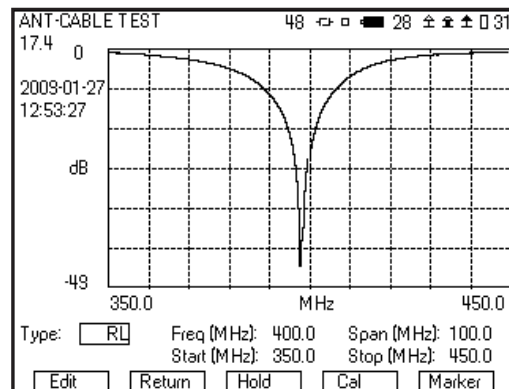
ANT-CABLE Test Screen Showing RL Versus Frequency
