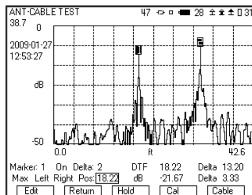
SWR Test Screen Showing DTF
